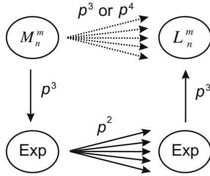
Fig. 4. Sketch of the MP to local translation schemes using the classical matrix–vector multiplication scheme (top, \mathcal{O}(p^4) ), using rotation based translation operators (top, \mathcal{O}(p^3) ) and using plane wave based translation operators (bottom).
